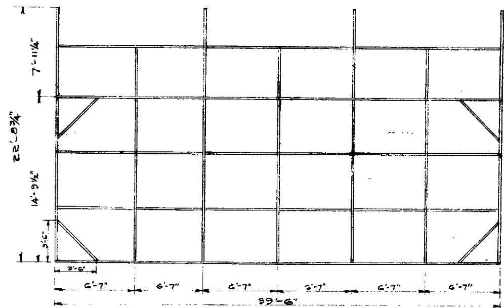
PLAN OF FRAME
