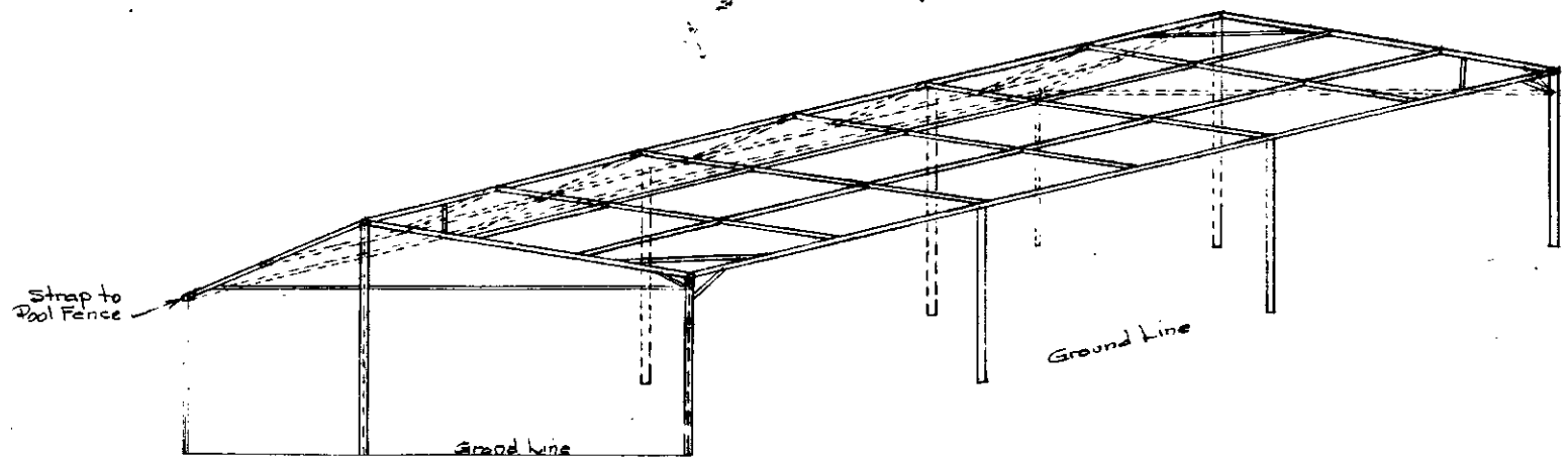
PERSPECTIVE Scale 1/4"=1'
