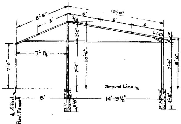
END ELEVATION Scale 1/4"=1'
